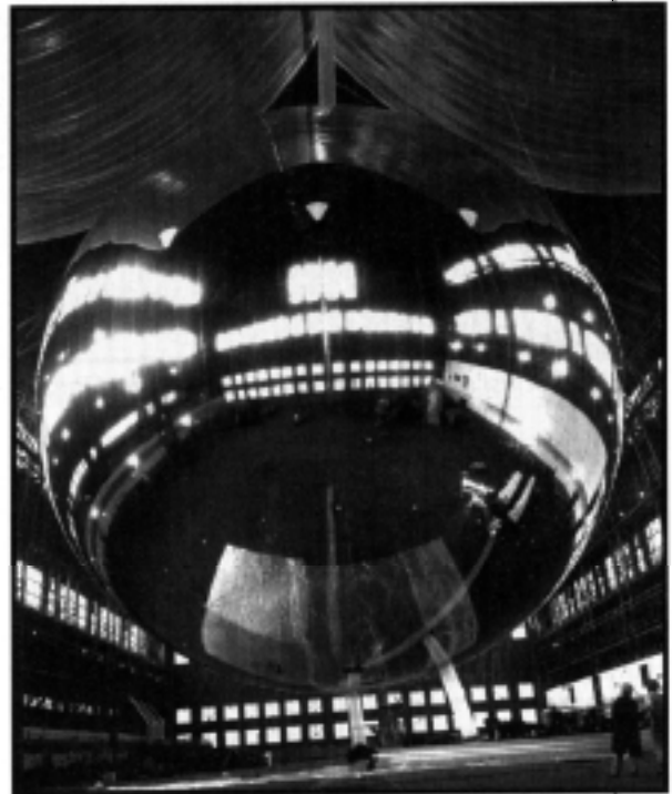
Fig. 1. Inflation test of PAGEOS – a 100-ft diameter satellite used in the National Geodetic Satellite Program.
