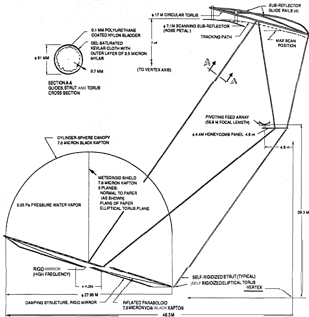
Fig. 7. Application of a large inflatable reflector for an Earth Sciences Geostationary Platform.
