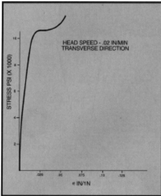
Fig. 5. A typical stress vs. strain curve for Mylar, illustrating the large modulus (slope) variations.
