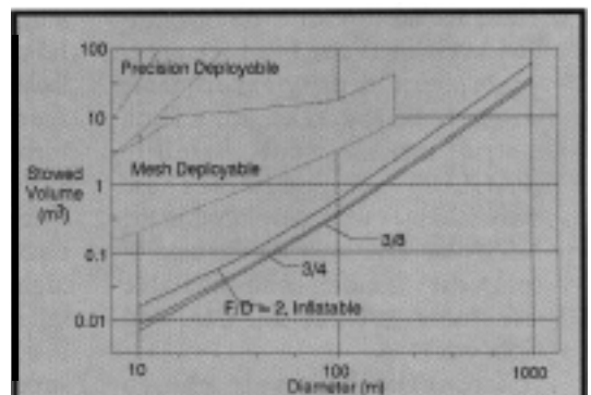
Fig. 4. Inflatables can generally be stored in volumes several orders of magnitude less than needed by competing structures.
