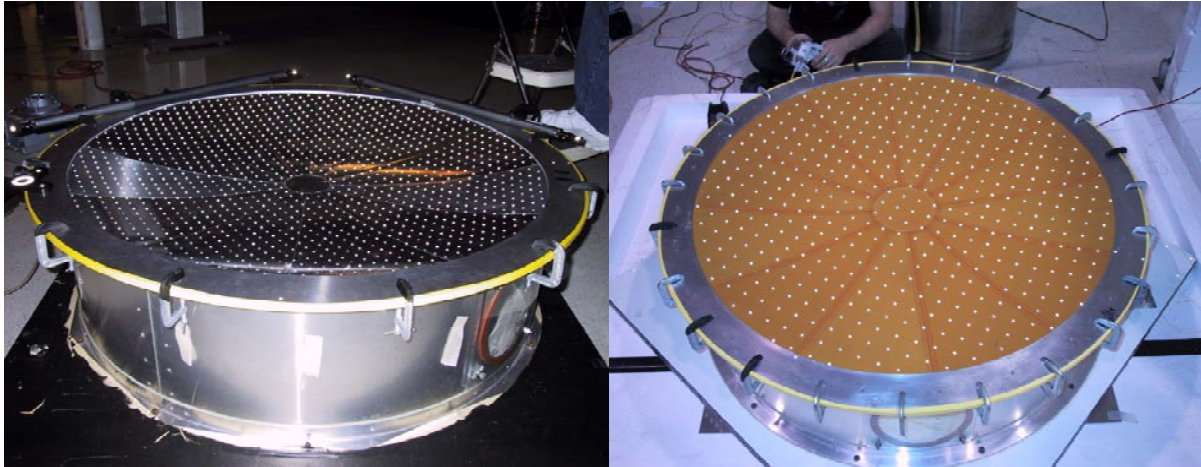
Figure 4. 1-Meter Test Articles.
