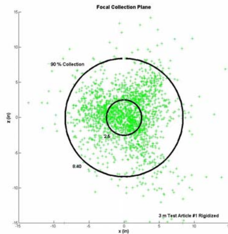
Figure 8. 3-Meter Test Reflector Collection Plot (Rigidized)
