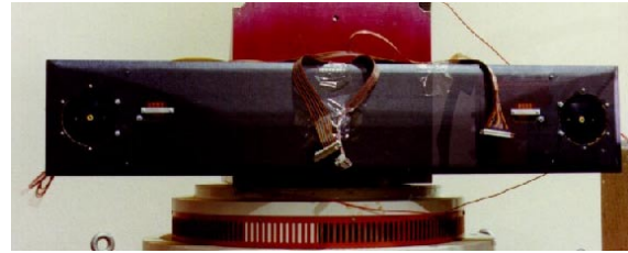
Figure 7. Random Vibration Tests
